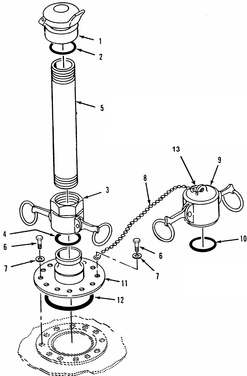
Figure 3. Vent Fitting Assembly.
